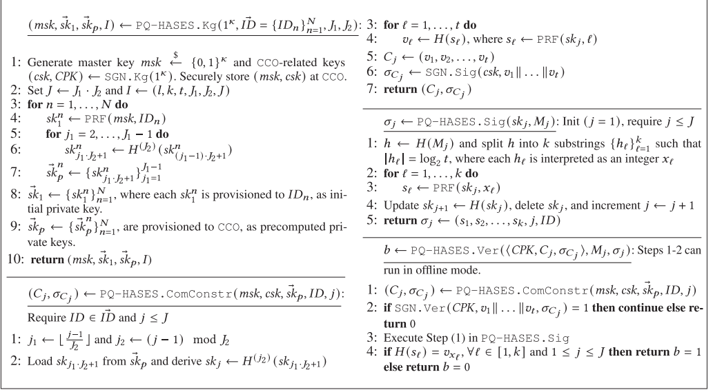
Fig. 1. The proposed PQ hardware-assisted digital signature with forward-security (PQ-HASES).
