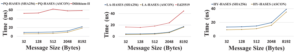
Fig. 5. Signature generation of HASES schemes and their counterparts on Commodity Hardware.
