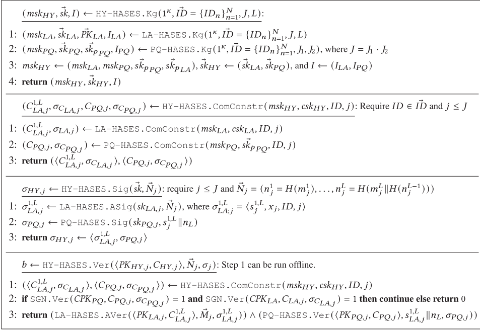
Fig. 4. The proposed hybrid hardware-assisted digital signature (HY-HASES).
