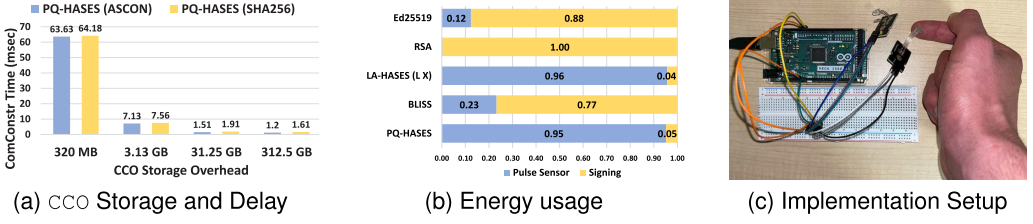
Fig. 6. CC0 Storage Impact on ComConstr Delay and Energy Usage of HASES schemes.
